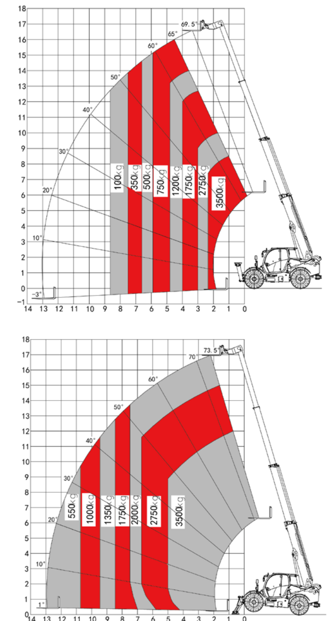
35THCJ17-CU1S Lifting diagram
