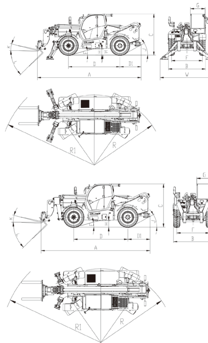
50THCJ17-CU1S Dimension
