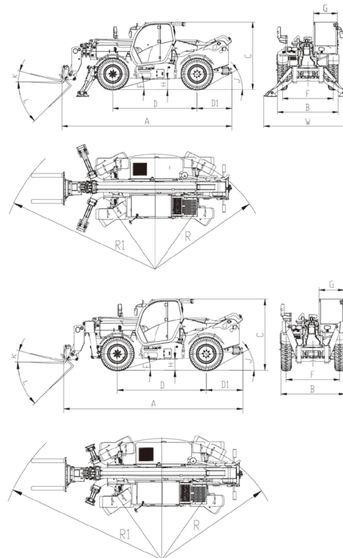
35THCJ17-CU1S Dimension
