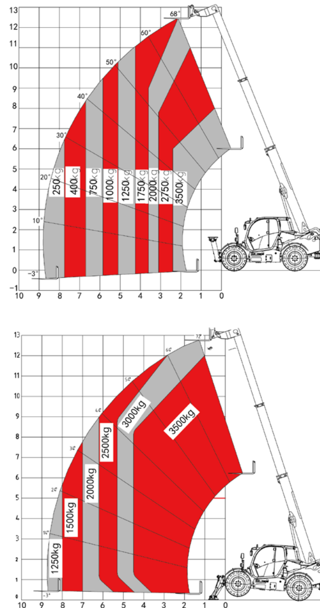
35THCJ13-CU1S Dimension
