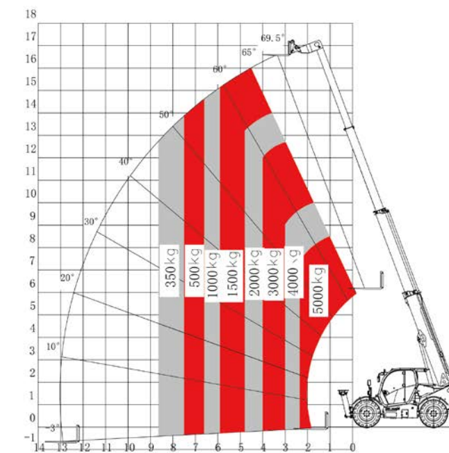
50THCJ17-CU1S Lifting diagram
