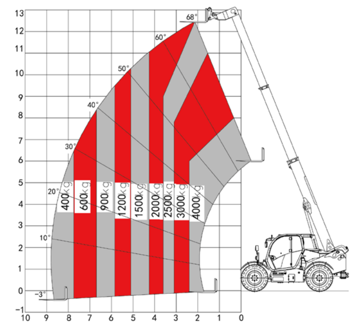
40THCJ13-CU1 Lifting diagram
